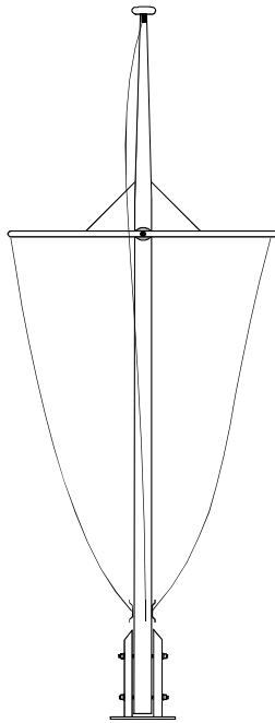
Flagpole with yardarm and tabernacle base
